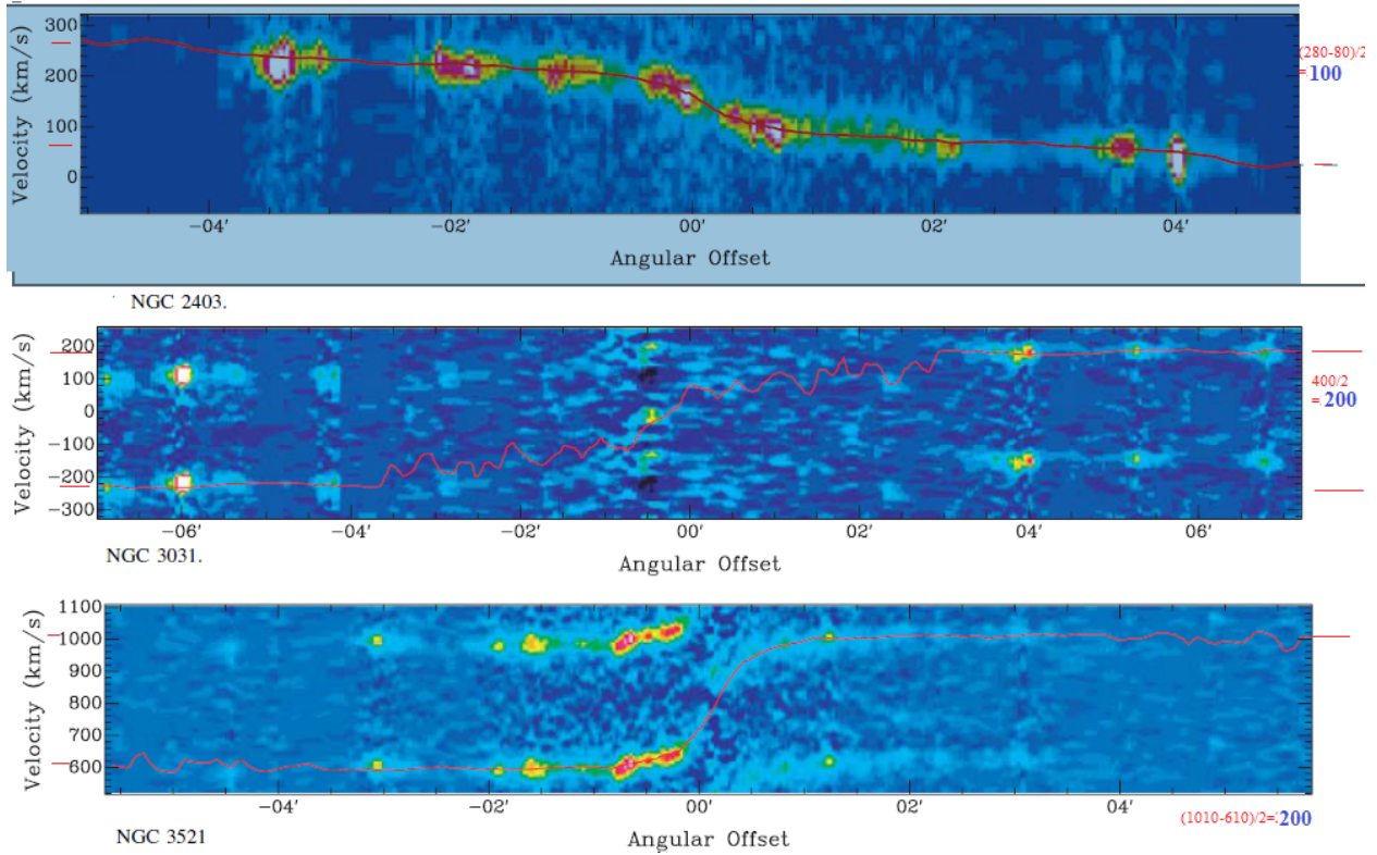
Figure A1 Velocity quantization In the Halos Of Nearby Galaxies (mostly 200km/sec)
