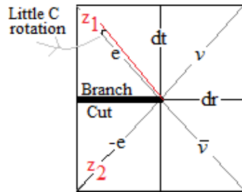
fig.3 Solutions to equation 5: eq7 quadrant II electron & III positron,
