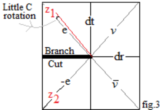
fig.3. for 45^\circ-45^\circ So two body (e,v) singlet \Delta S = 1/2 - 1/2 = 0 component so pairing interaction (sect.4.5). Also ortho \Delta S = 1/2 + 1/2 = 1 making 2 body (at r=r_H ) S=1 Bosons and so a field theory. Note we also get these Laplacians characteristic of the Boson field equations by those 45^\circ+45^\circ rotations so eq.16 implies Bosons accompany our leptons (given the \delta z' ), so these leptons exhibit "force" .
