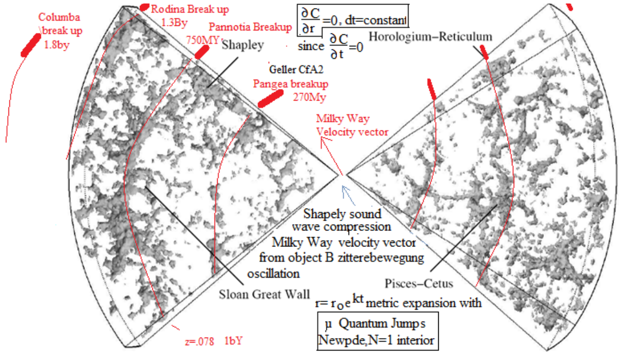
Fig1 Above are the \frac{\partial C}{\partial r} , dt constant N=2 (observable internal QMS jumps in fig 1). A QMS (quantum mechanical system) state region jumps all at once as seen by the outside fractal larger observer so it should do that for the inside ( r_H ) observer as well. Because of that the disturbance appears to propagate from any given point at speed c even though it actually happened simultaneously everywhere at once in the QMS. Thus we see these Sloan and Margaret Geller Great Walls that appear to be centered on our own position (corrected for our own galaxy's proper motion). But they really aren't centered here. It's just that the jump(s) occur all at once over the entire QMS.
