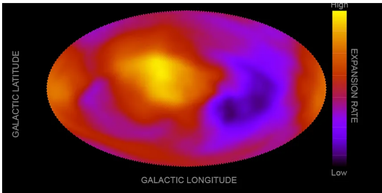
Fig1 Above are the \frac{\partial C}{\partial r} , dt constant N=2 (observable internal QMS jumps in fig 1). A QMS (quantum mechanical system) state region jumps all at once as seen by the outside fractal larger observer so it should do that for the inside ( r_H ) observer as well. Because of that the disturbance appears to propagate from any given point at speed c even though it actually happened simultaneously everywhere at once in the QMS. Thus we see these Sloan and Margaret Geller Great Walls that appear to be centered on our own position (corrected for our own galaxy's proper motion). But they really aren't centered here. It's just that the jump(s) occur all at once over the entire QMS.
