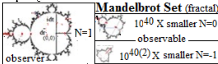
fig1. If N is the 'observers' fractal
