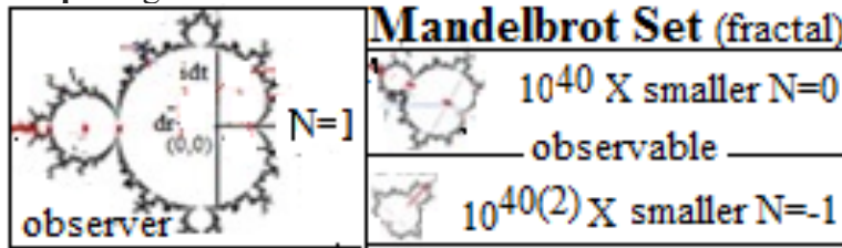
fig1 Zoom done at Fiegnbaum pt.
