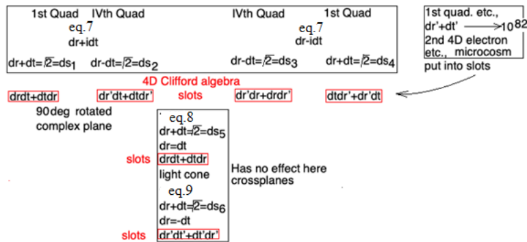
Fig.8 These added cross term eq.11a objects (1.11) extend eigenvalue equation 11 from merely saying 1+1=2 all the way to the number 10^{82} .
