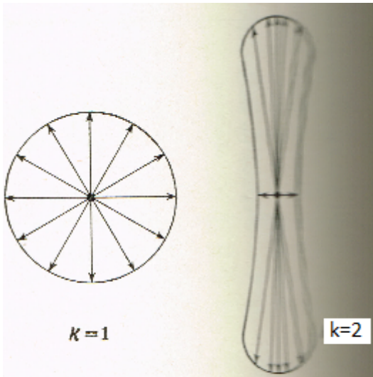
EField Representation of the electric field intensity about a stationary and a rapidly moving charge.
