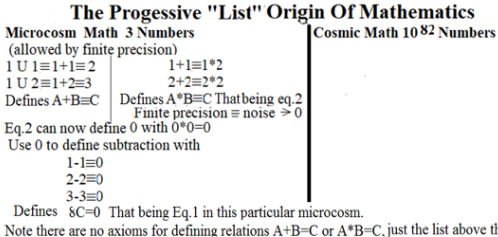
Fig.7 in that particular microcosm. There are no postulated rings or fields here either.
