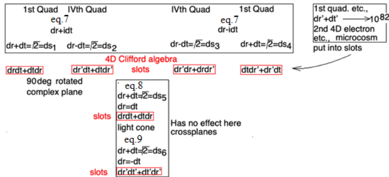
Fig.6 These added cross term eq.1.11a objects (1.11) extend eigenvalue equation 11 from merely saying 1+1=2 all the way to the number 10^{82} .
