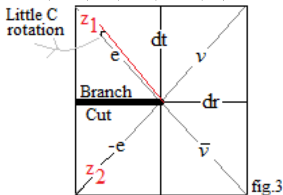
fig.3. for 45^\circ - 45^\circ So two body (e,v) singlet \Delta S = 1/2 - 1/2 = 0 component so pairing interaction (sect.4.5). Also ortho \Delta S = 1/2 + 1/2 = 1 making 2 body (at r=r_H ) S=1 Bosons and so a field theory. Note we also get these Laplacians characteristic of the Boson field equations by those 45^\circ + 45^\circ
