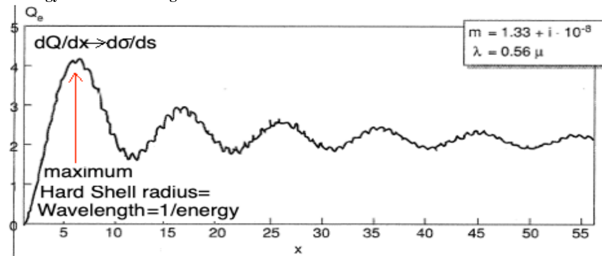
Fig6 Analogy to Mie scattering
